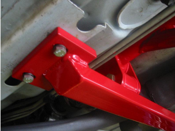
Image 1- Cross Brace Mounted in Place with 8mm x 30mm Bolts
