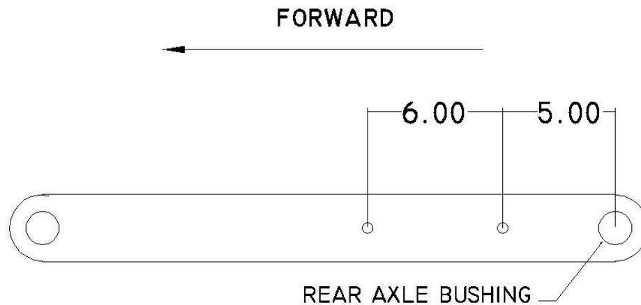
LOWER CONTROL ARM DRILLING DIAGRAM
