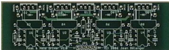
4 way peak&hold low-z driver board
