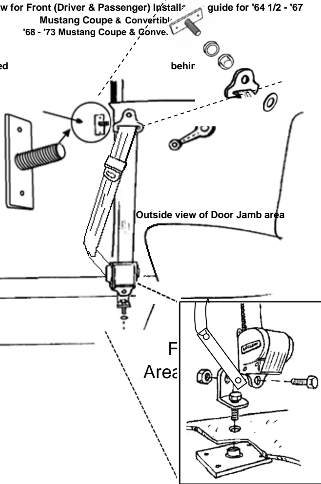
Detail showing anchor plate installed underneath floor (beneath car).
