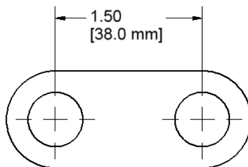
DRILLING TEMPLATE
