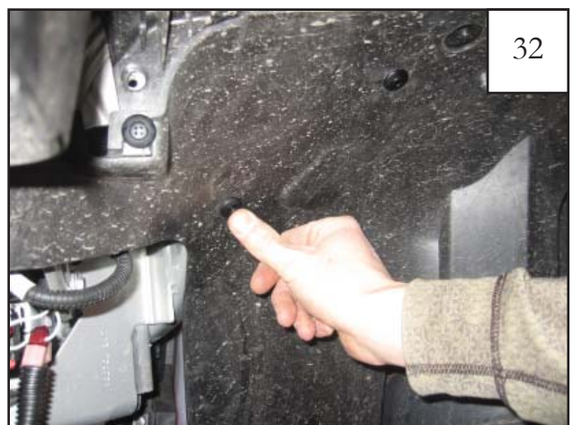
Install a supplied Plastic Phillips Head Tuf-lok in hole located towards the front of the splash shield.
